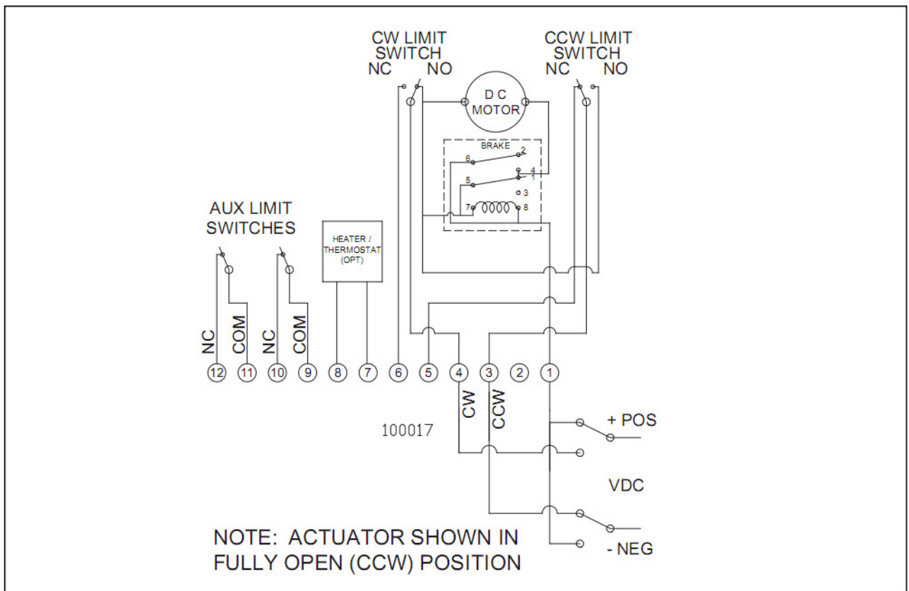
Figure 3B LUF Series DC Wiring
