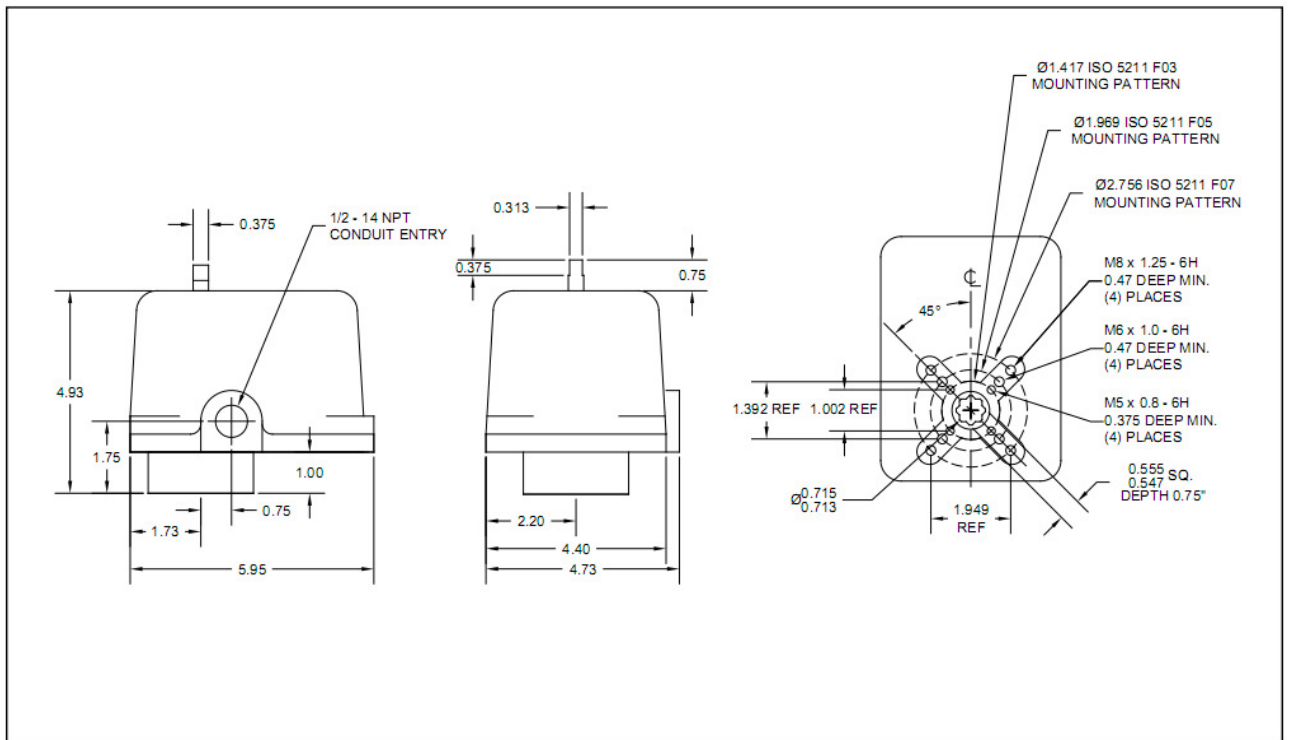
Figure 2B Dimensions, Female output (optional)
