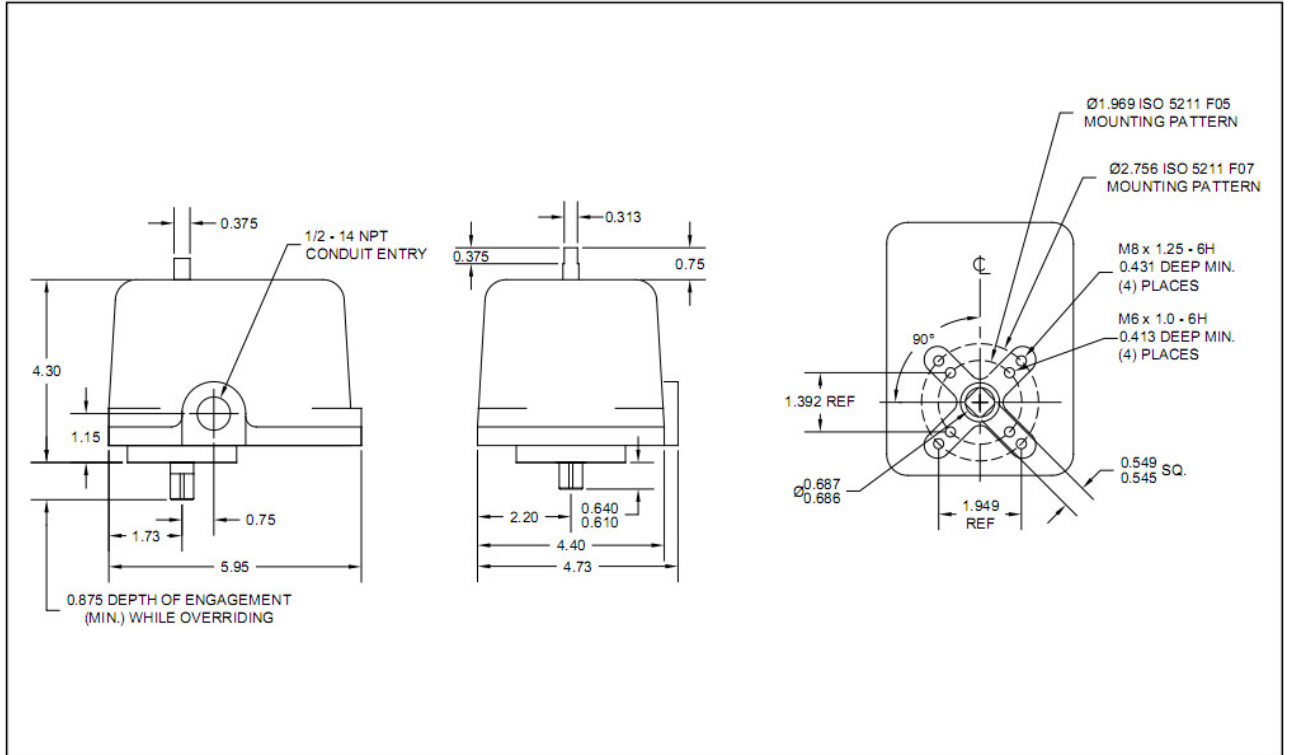
Figure 2A Dimensions, Male output (standard)
