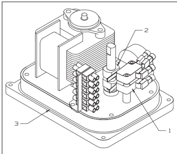
Figure 1 Parts Identification
